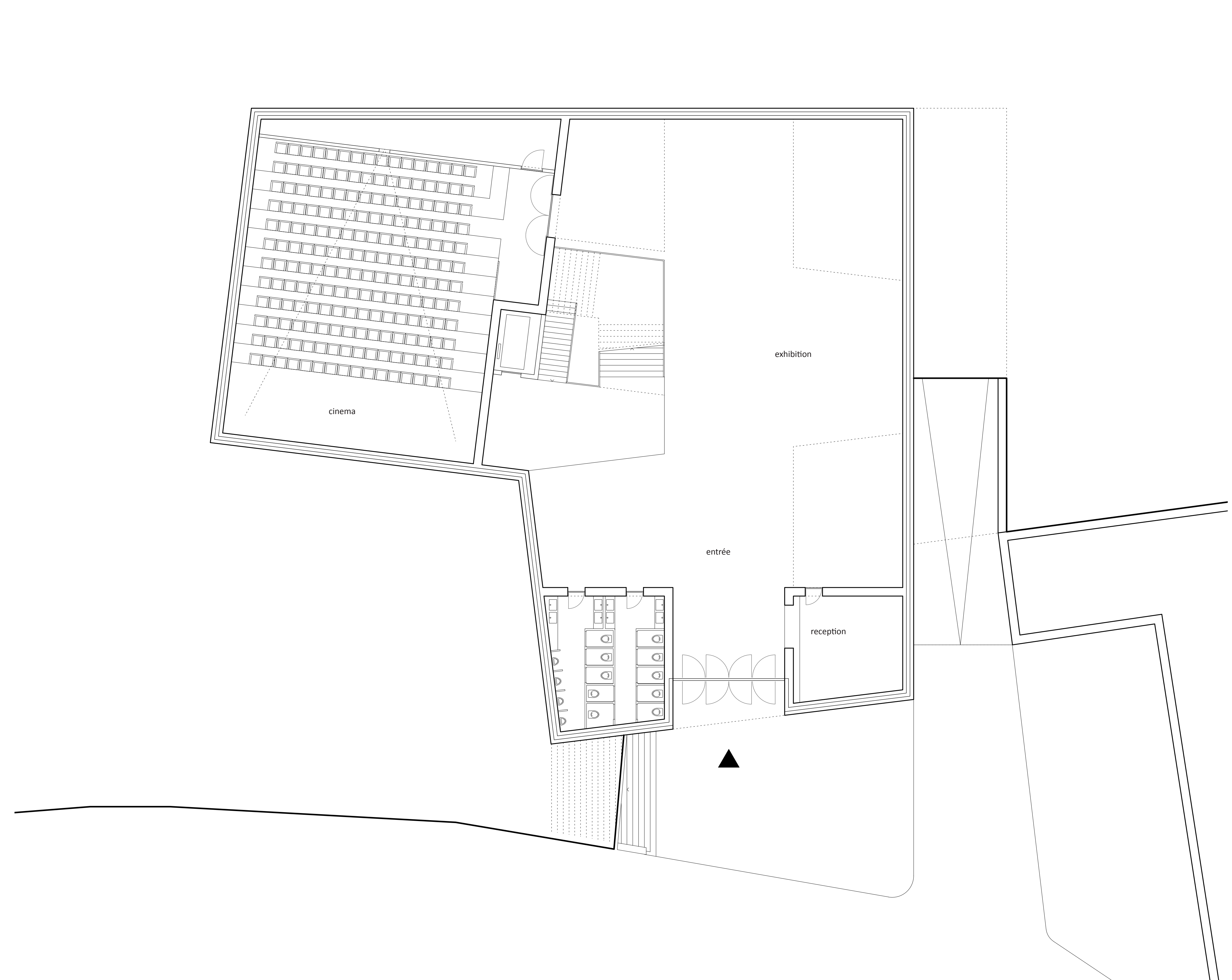
layout ground floor, M1:100
