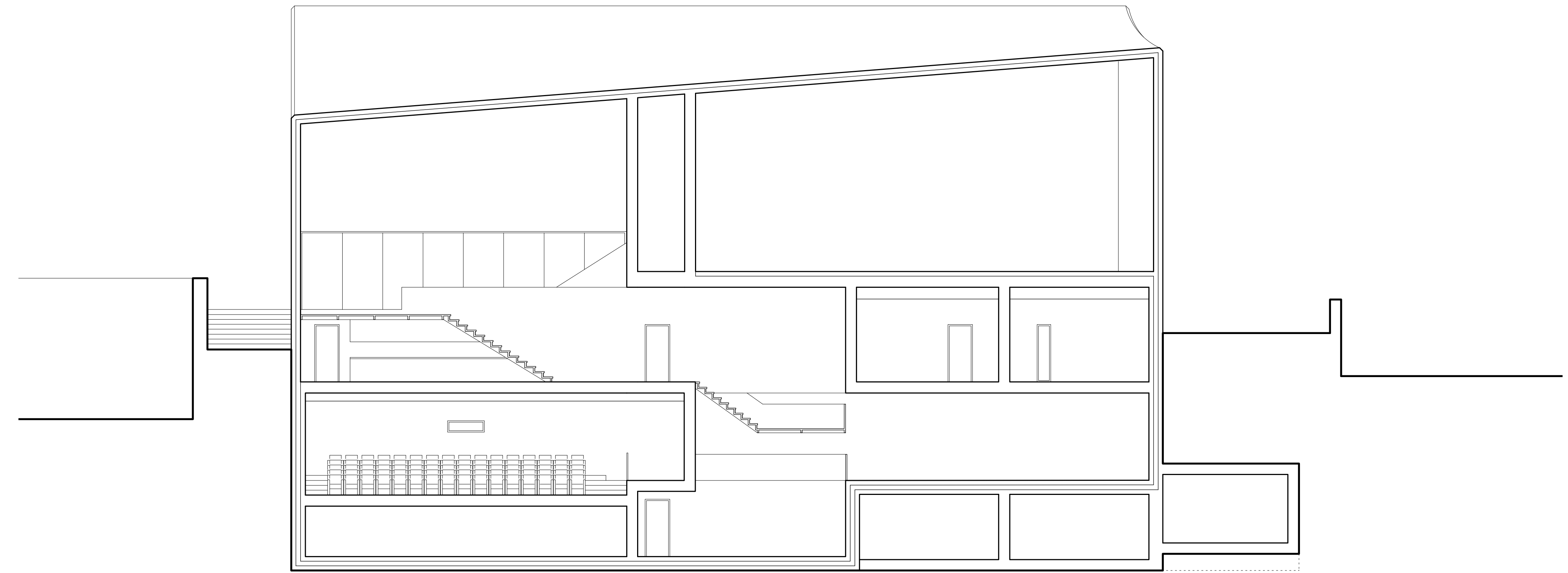
section B-B, M1:100
