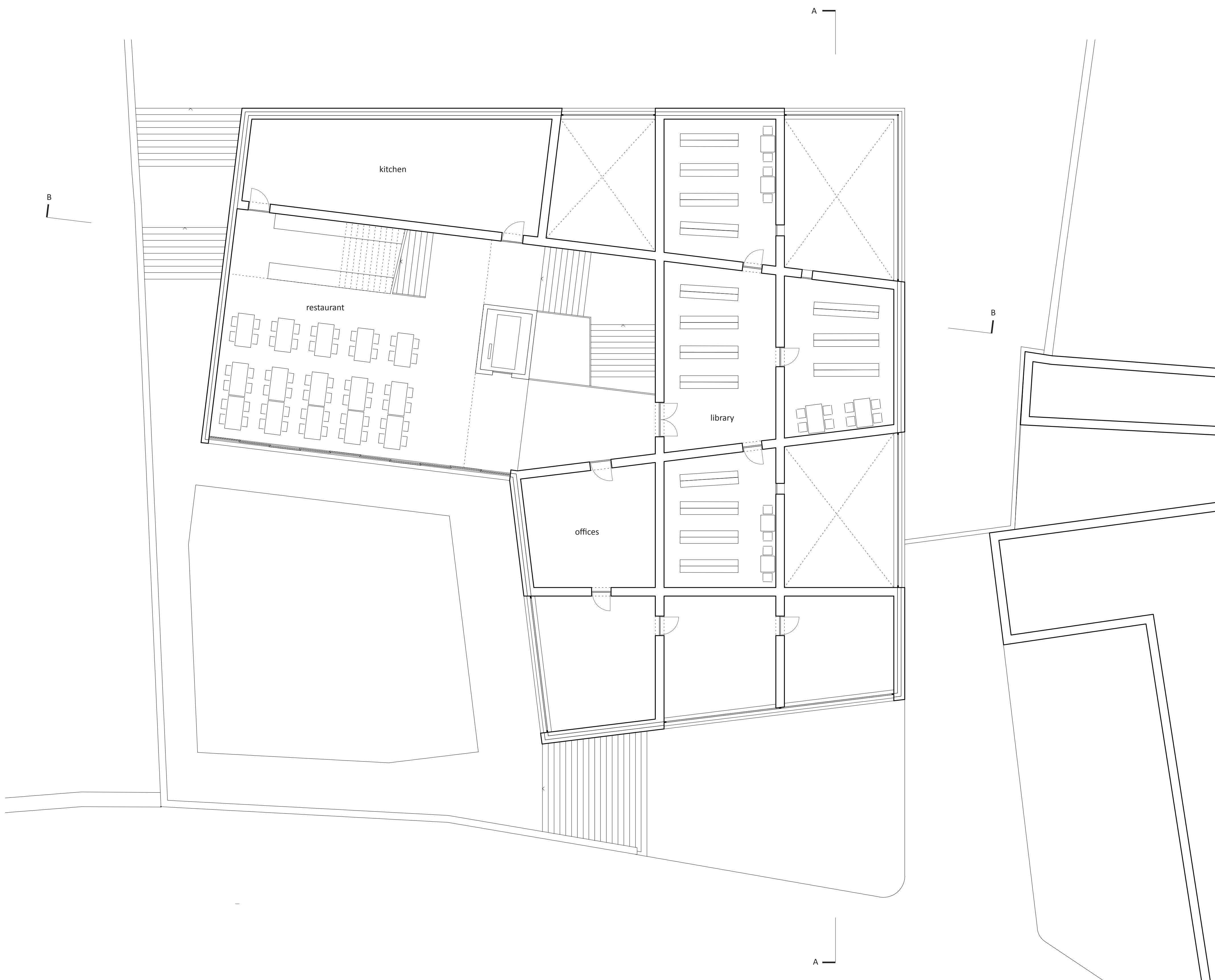
layout first floor, M1:100
