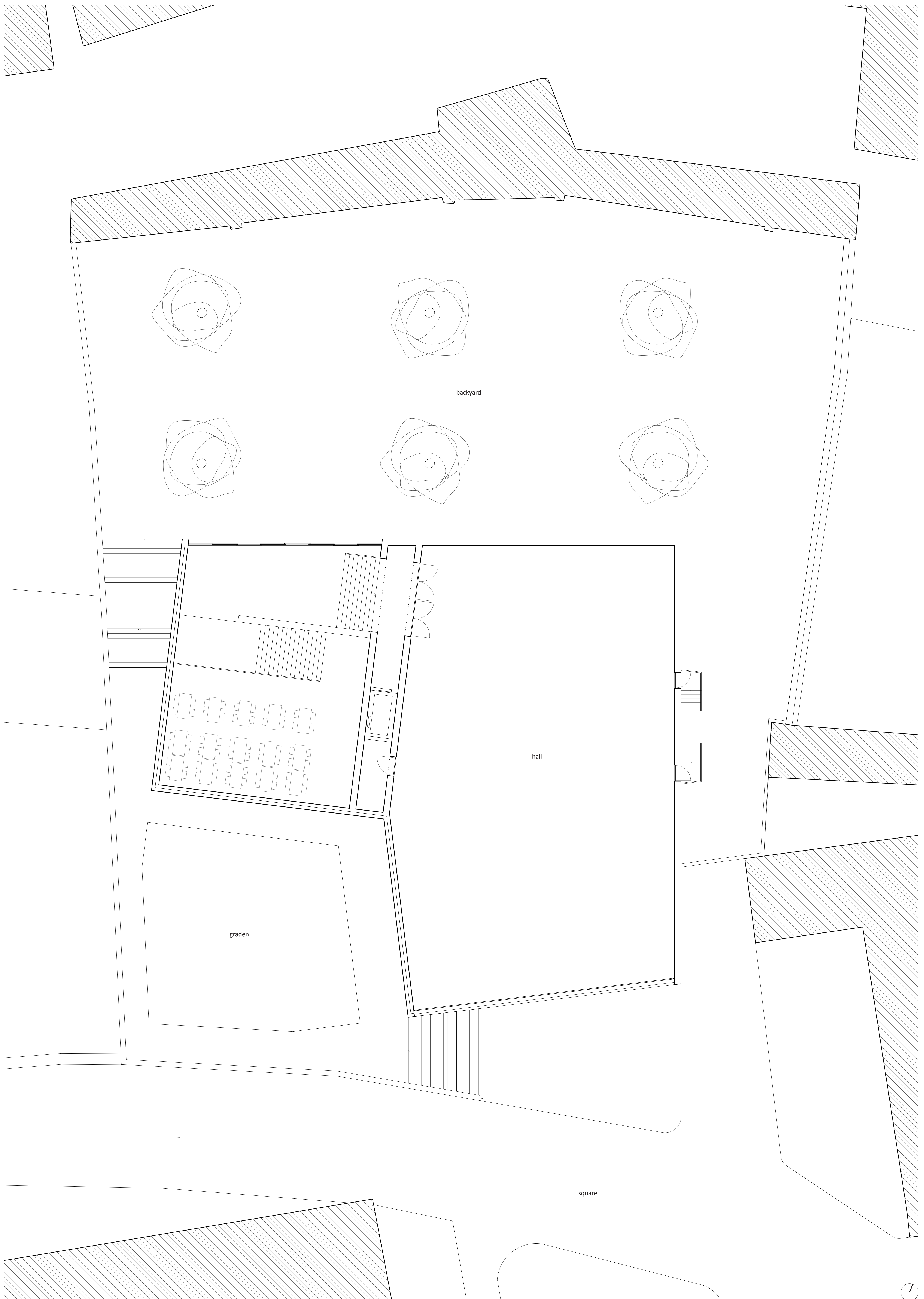
layout second floor, M1:100
